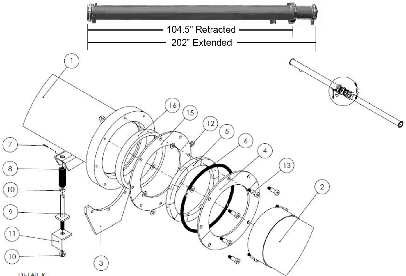
DETAIL K
